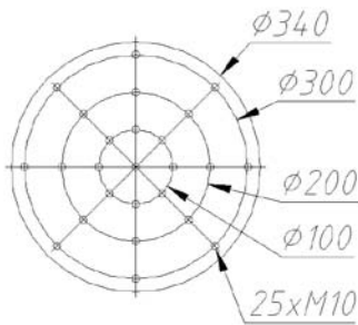
Armature insert pattern
