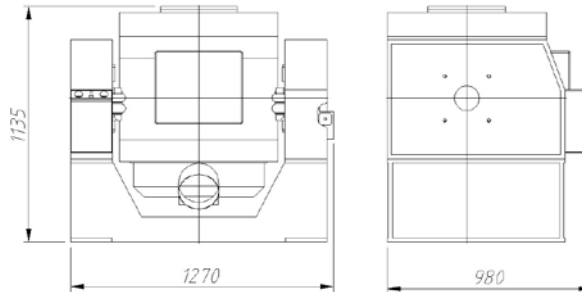
Shaker body
